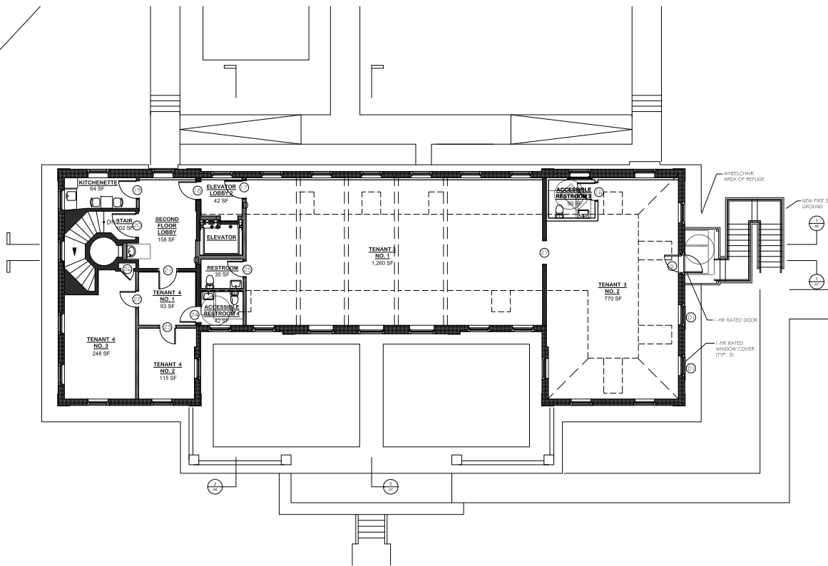
1 PROPOSED SECOND FLOOR PLAN A2 SCALE: 1/8" = 1'-0"
